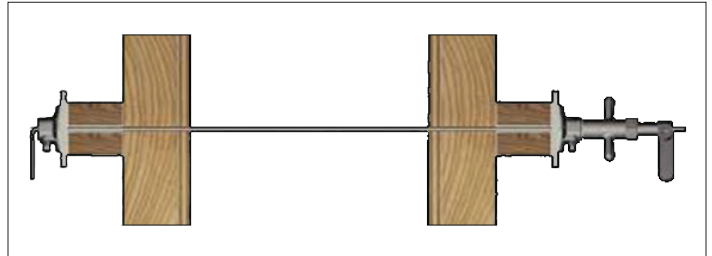
Pencil Rod and Rod Clamps ties formwork together and holds it securely during concrete placement.
